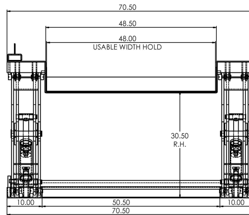
END VIEW-RAISED POSITION
