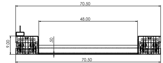
END VIEW-LOWERED POSITION
