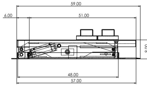
SIDE VIEW-LOWERED POSITION
